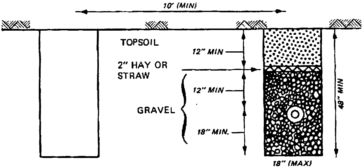
Figure 3-32. Seepage Ditch
